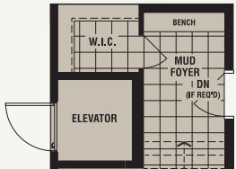
PARTIAL GROUND FLOOR PLAN W/ OPT. ELEVATOR
