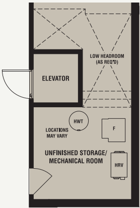
PARTIAL FINISHED BASEMENT PLAN W/ OPTIONAL ELEVATOR (SIMILAR FOR GUEST SUITE OPTION)
