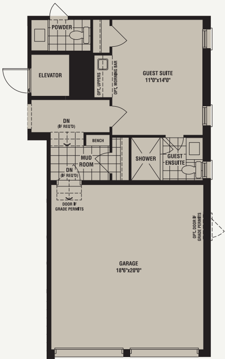
GROUND FLOOR GUEST SUITE OPTION W/ ELEVATOR +219 SQ. FT.
