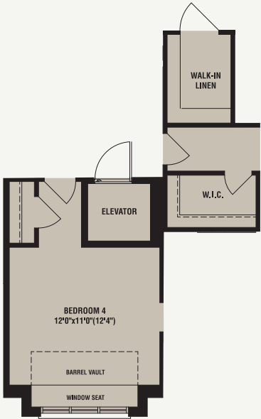
PARTIAL GROUND FLOOR PLAN W/ OPTIONAL ELEVATOR
