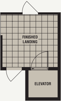
PARTIAL BASEMENT PLAN W/ OPTIONAL ELEVATOR (SIMILAR FOR GUEST SUITE & FINISHED BASEMENT OPTIONS)
