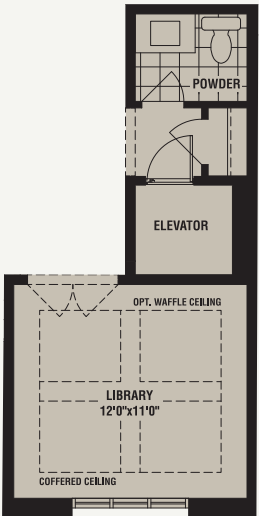
PARTIAL GROUND FLOOR PLAN W/ OPTIONAL ELEVATOR
