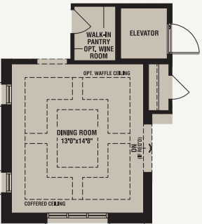
PARTIAL GROUND FLOOR PLAN / OPTIONAL GROUND FLOOR PLAN W/ GUEST SUITE - W/ OPT. ELEVATOR
