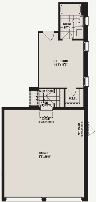
GROUND FLOOR GUEST SUITE OPTION +199 SQ. FT.
